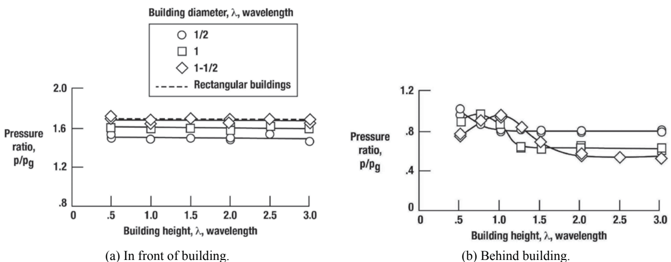
Figure 9.96. Pressure ratio on the ground in front of and behind cylindrical building due to sonic booms at an angle of 30^\circ to the building and 60^\circ to the ground (ref. 9.57).
