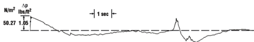
(a) Measured on USS Salinan , Overhead Conditions: Velocity = 2210 m/sec and Altitude = 63,422 meters.
