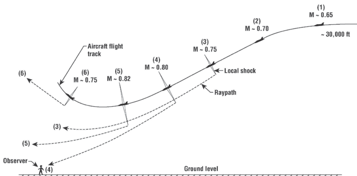
Figure 3.32. Schematic illustration of local shock waves and ray paths emanating from an aircraft in a 20° dive at Mach < 1.0.
