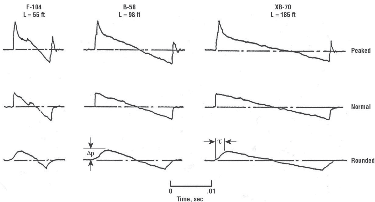
Figure 2.29. Influence of atmosphere on boom signatures from different size aircraft (adapted from ref. 2.25).
