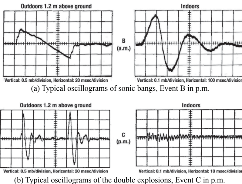
Figure 9.141. The waveforms of typical sonic bangs and explosions as measured outdoors and indoors (adapted from ref. 9.85).
