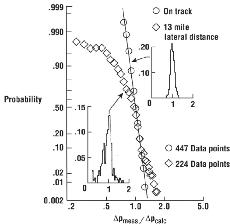
Figure 2.40. Effect of lateral distance on sonic boom variability; XB-70 at Mach 1.8–2.5 at 60,000 feet (adapted from ref. 2.15).
