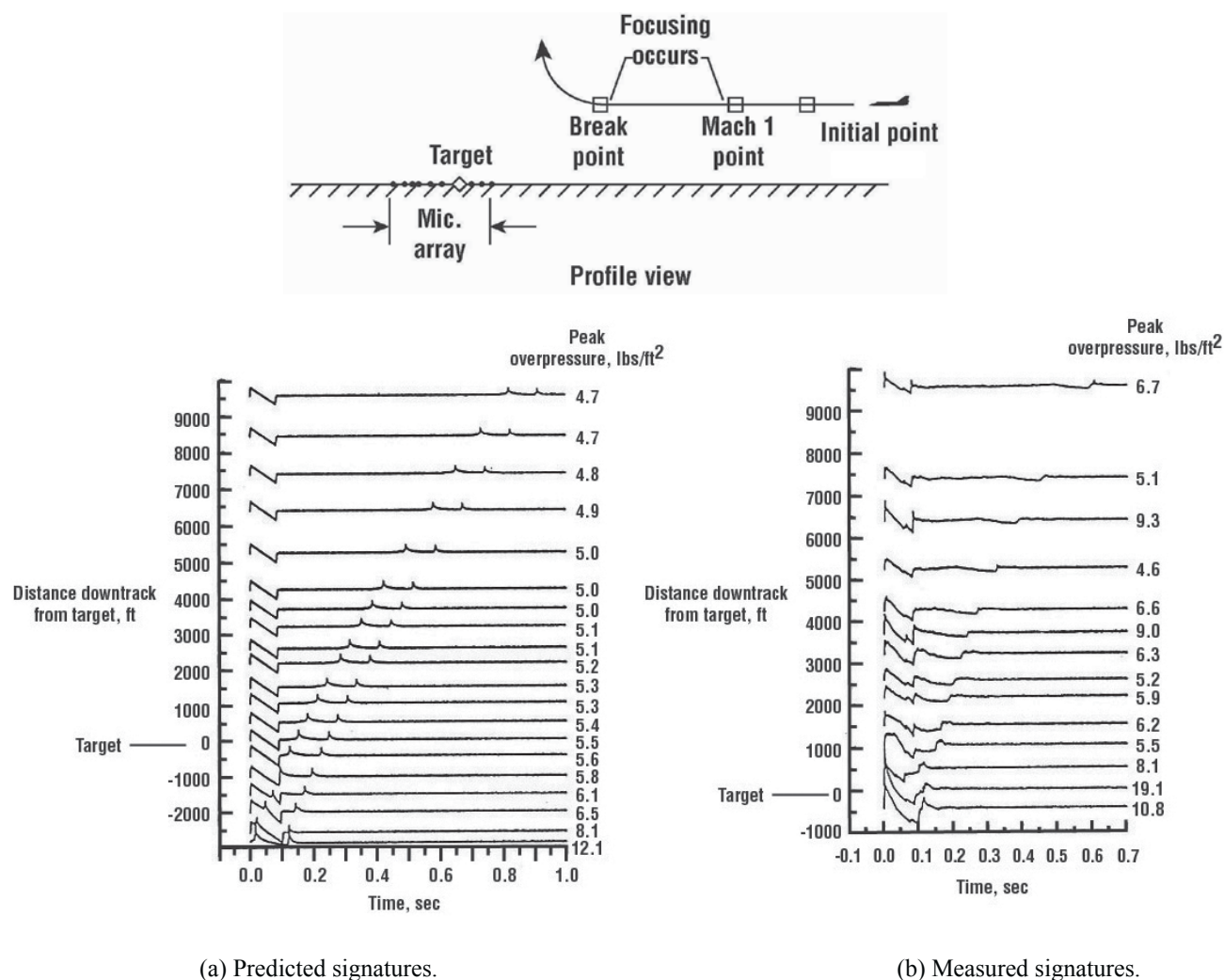
Figure 3.11. Comparison of on-track predicted and measured sonic boom signatures during transition flight, level acceleration of F-16 from Mach 0.9 to Mach 1.2 at 10,000 ft (adapted from ref. 3.6).
