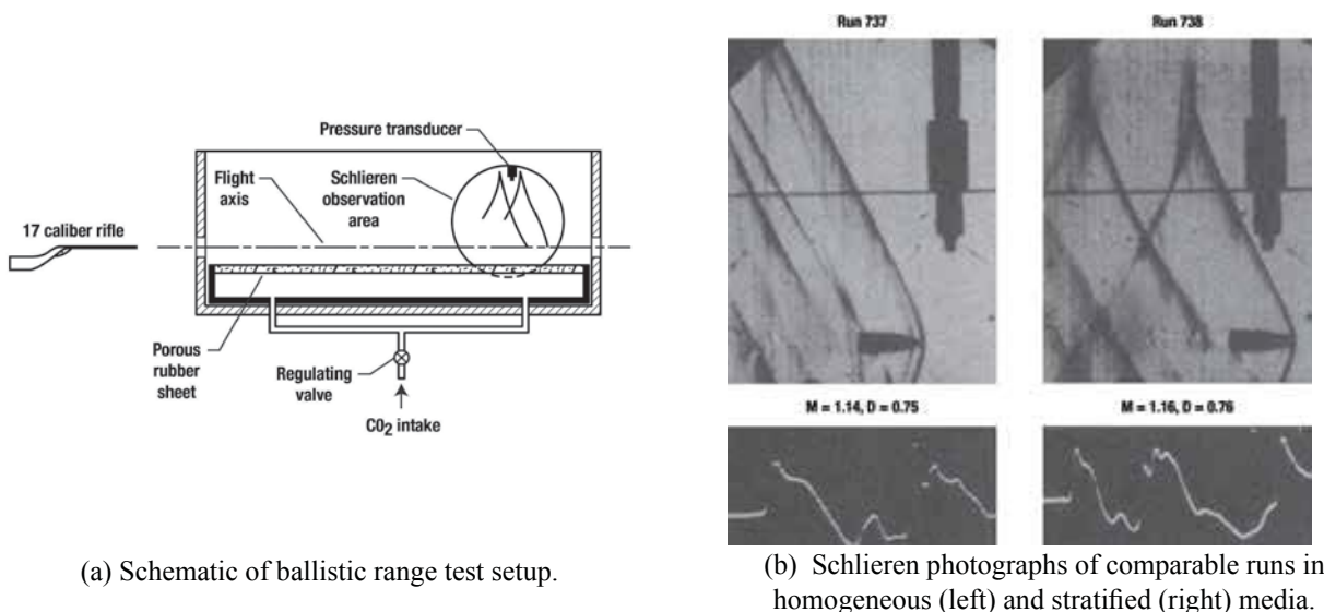
Figure 9.63. Schematic diagram and test results of experimental apparatus to measure sonic boom focusing due to atmospheric refraction (adapted from ref. 9.38).
