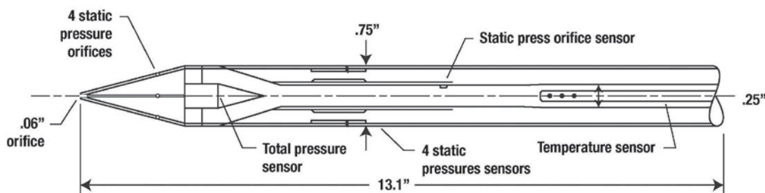
Figure 9.15. Schematic of conical probe with total temperature gage to provide free-stream pressure, Mach number, angle-of-attack, and free-stream velocity, static temperature, and speed of sound (ref. 9.14).
