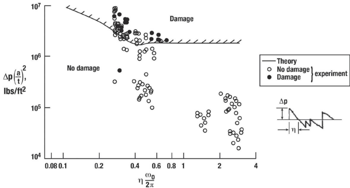
Figure 8.17. Summary of window-glass breakage due to sonic booms (refs. 8.22, 8.23, 8.7, and 8.2).
