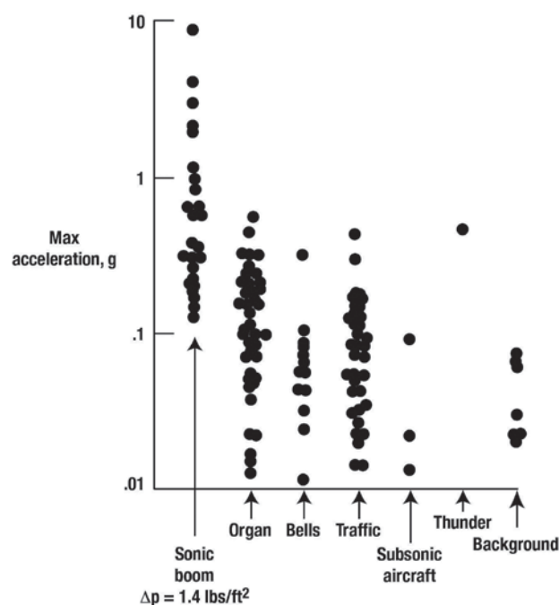
Figure 8.21. Response of cathedral windows to transient pressures (ref. 8.2).
