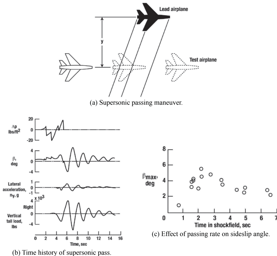
Figure 8.45. Formation flying at supersonic speeds (adapted from ref. 8.94).
