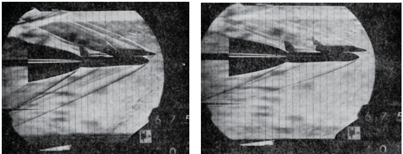
(a) Launch configuration with simulated plume (Mach 3).
