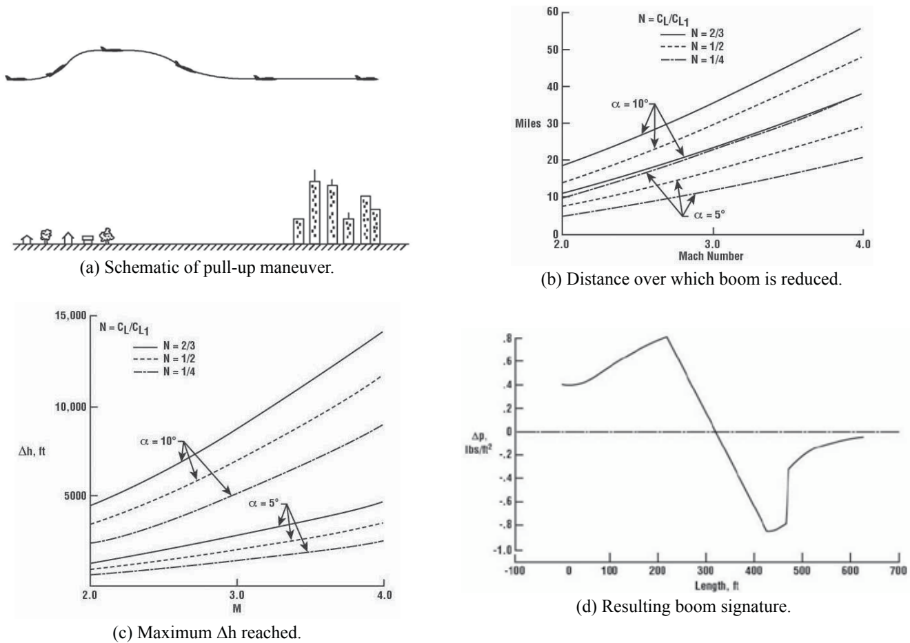
Figure 5.10. Local reduction of sonic boom by maneuvering aircraft (adapted from ref. 5.2).
