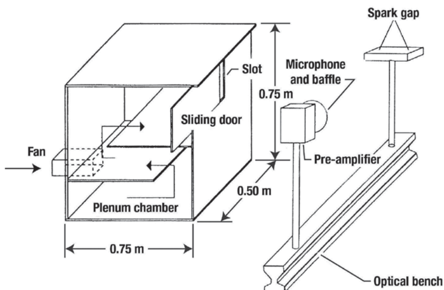
Figure 9.56. Arrangement of the experiment – plane jet source, spark source (without the parabolic reflector), and receiver. The dimensions shown are in meters (adapted from ref. 9.31).
