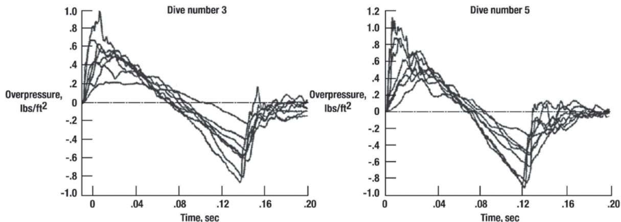
Figure 8.24. Ground-level sonic boom measurements from the F/A-18B aircraft in a supersonic low-boom dive maneuver (ref. 8.35).
