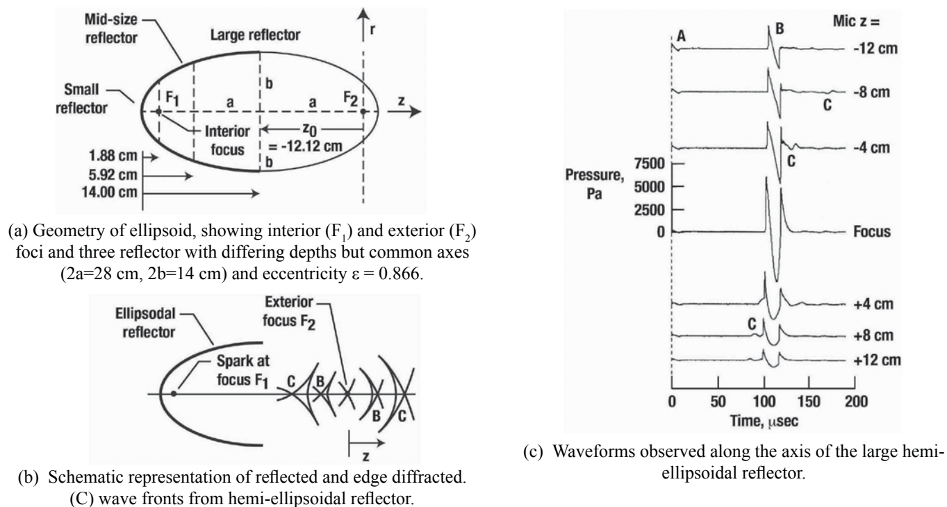
Figure 9.70. Laboratory test setup and results from spark and ellipsoidal mirror focus boom experiment (ref. 9.42).
