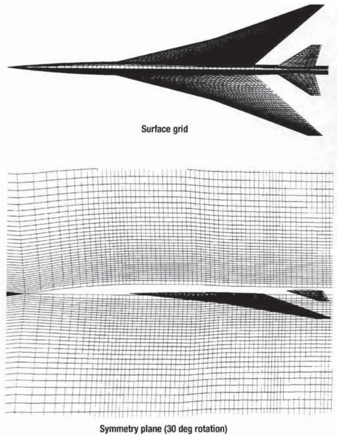
Figure 7.52. HFL04 computational grid (ref. 7.35).
