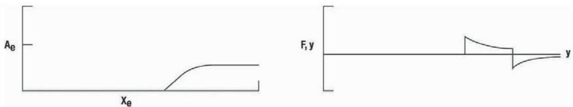
Figure 7.44. Equivalent area and F-function for an isolated nacelle (ref. 7.32).
