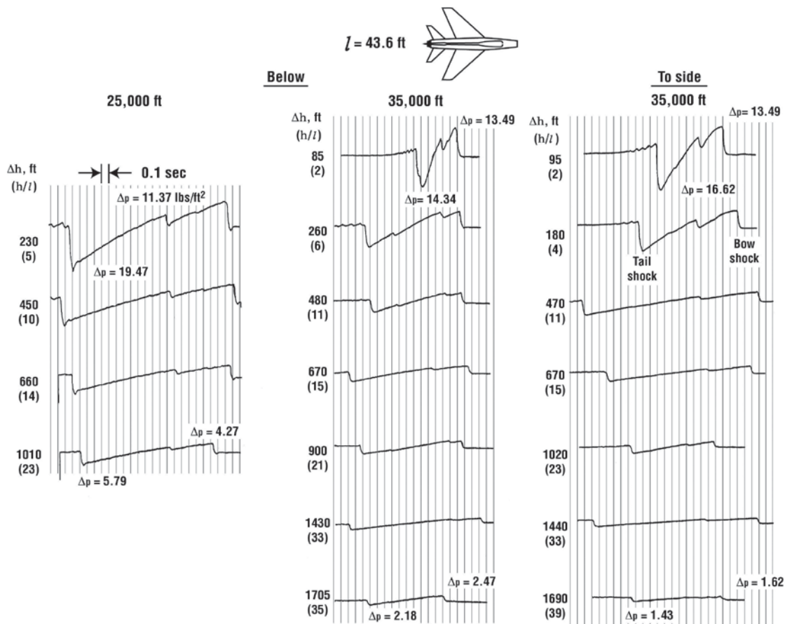
Figure 4.3. In-flight flow-field signatures measured below and to the side of an F-100 aircraft at Mach 1.05 (adapted from ref. 4.2).
