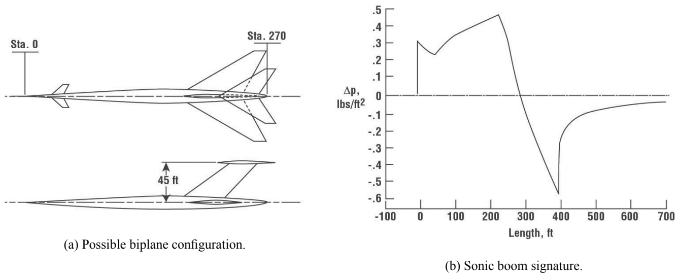
Figure 5.27. Possible biplane configuration and predicted boom signature, Mach 1.5 at 40,000 ft, l = 290 ft, w_{\text{cruise}} = 320,000 lbs, 250 PAX, 2800 mile range (adapted from ref. 5.2).
