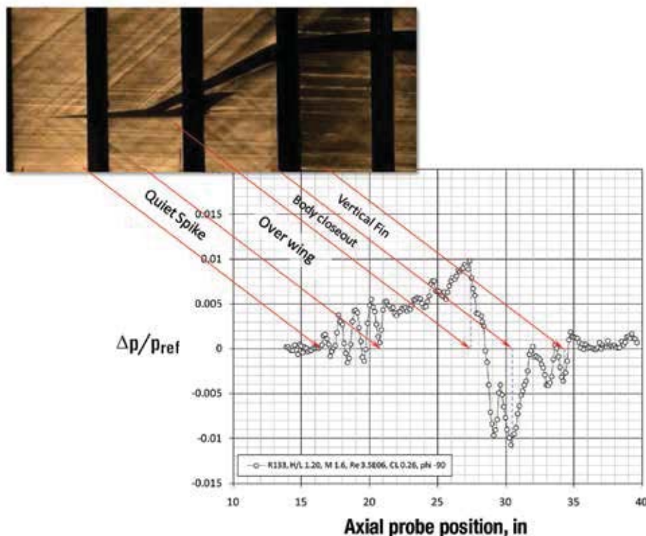
Figure 9.29. Schlieren and near-field signature data of Gulfstream wind-tunnel model with blade mount (ref. 9.20).
