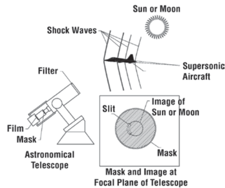
(b) Schlieren setup for aircraft in flight.
