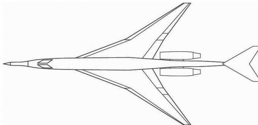
Figure 7.39. Boom optimized configuration plus small manual modifications (adapted from ref. 7.29).
