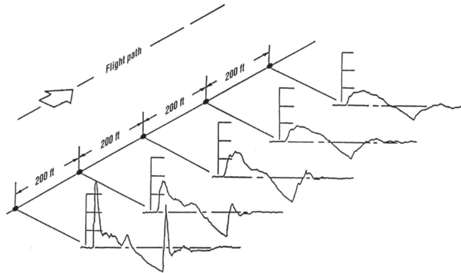
Figure 2.17. Variations in sonic boom signatures along ground track for steady-level flight (adapted from ref. 2.18).
