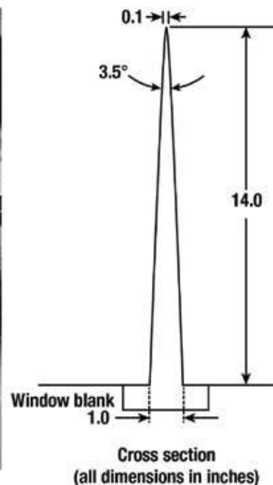
Figure 9.24. RF 1.0 pressure rail mounted on the aft window blank at the NASA ARC 9 - by 7-foot Supersonic Wind Tunnel (ref. 9.16).
