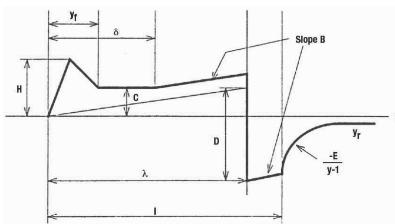
Figure 7.10. Combination flat-top and ramp signature (ref. 7.18).
