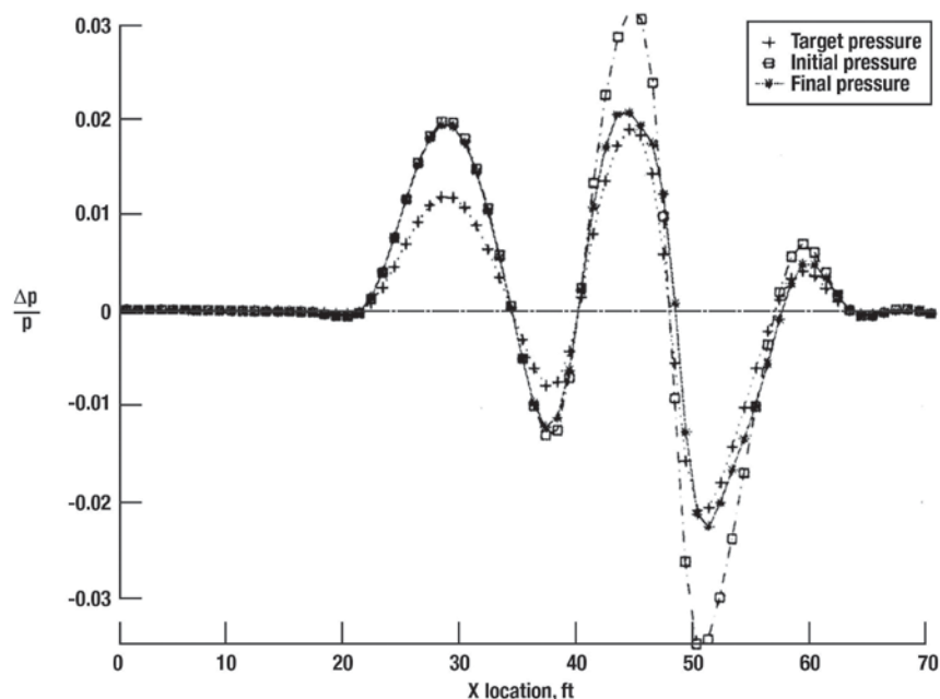
Figure 7.26. Sonic boom reduction: target, initial, and final near-field pressure distribution after 50 design cycles, Mach = 1.5 , \alpha = 1.62^\circ , lift not constrained (adapted from ref. 7.24).
