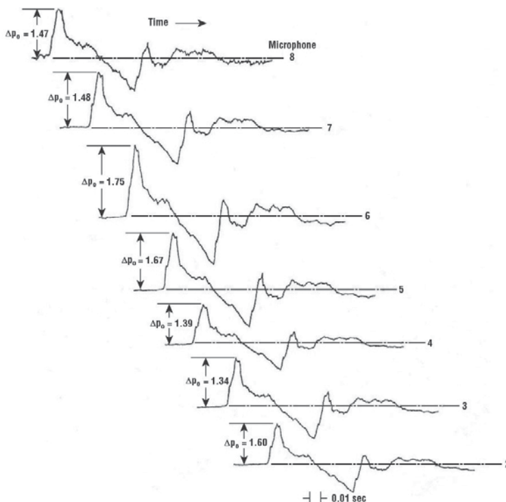
Figure 2.16. F-104 Sonic boom signatures from seven microphones grouped within a one-square foot area on ground, Mach 1.52 and altitude of 41,200 feet, \Delta p_0 is in lbs/ft 2 (adapted from ref. 2.17).
