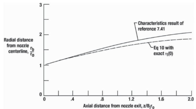
(c) M_j = 3.0 , M_\infty = 3.0 , p_j/p_\infty = 12.23 , nozzle wall angle = 12.5^\circ , boattail angle = 0^\circ .
