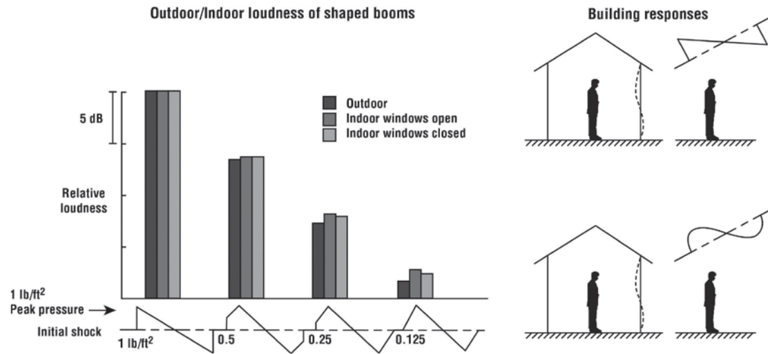
Figure 5.2. Sonic boom loudness and building response (adapted from ref. 5.1).
