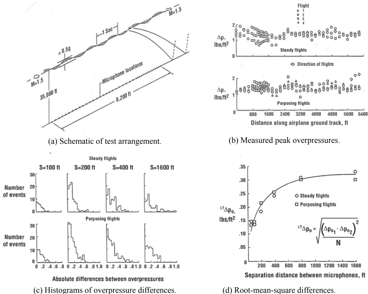
Figure 2.24. Influence of an F-106 aircraft's motion on sonic boom signatures at ground. The aircraft was flying over EAFB at Mach 1.5 and an altitude of 35,000 feet (adapted from ref. 2.15).
