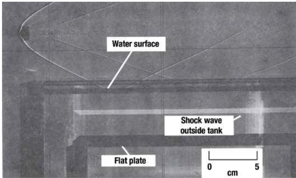
Figure 9.82. Shadowgraph picture of model flying over Plexiglas water-filled tank at Mach 2.7 in air M_{\text{water}} = 0.6 (ref. 9.47).
