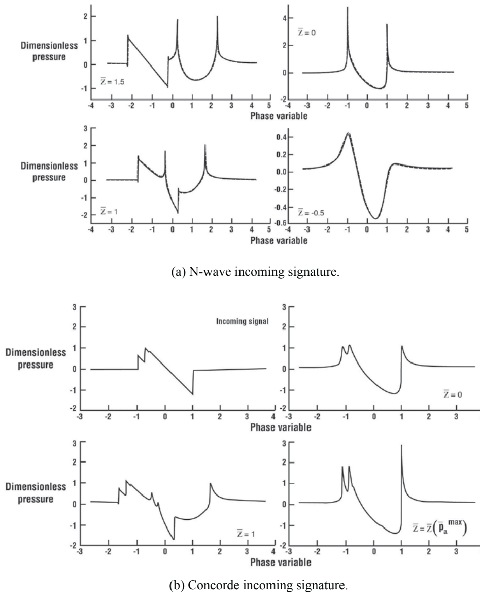
Figure 3.17. Influence of incoming sonic boom signature on focus boom during transition flight (ref. 3.21).
