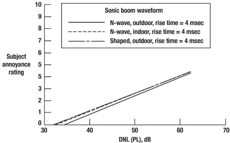
Figure 9.129. Effect of sonic boom waveform shape on annoyance versus day-night average sound level based on the perceived level noise metric (ref. 9.76).
