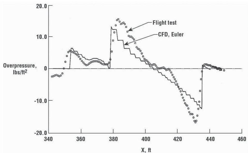
Figure 4.15. Comparison of measured and predicted in-flight SR-71 boom signature (adapted from ref. 4.23).
