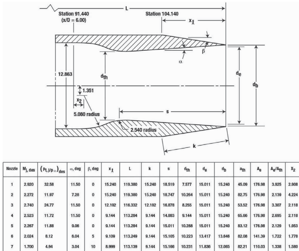
Figure 7.77. Details of nozzles. All dimensions are in cm except as noted. Areas are in \text{cm}^2 (ref. 7.42).
