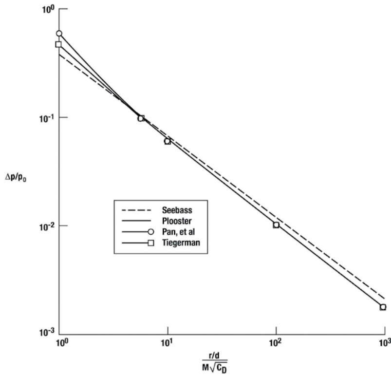
Figure 6.37. Variation of \Delta p/p_o with r/d/M\sqrt{C_D} .
