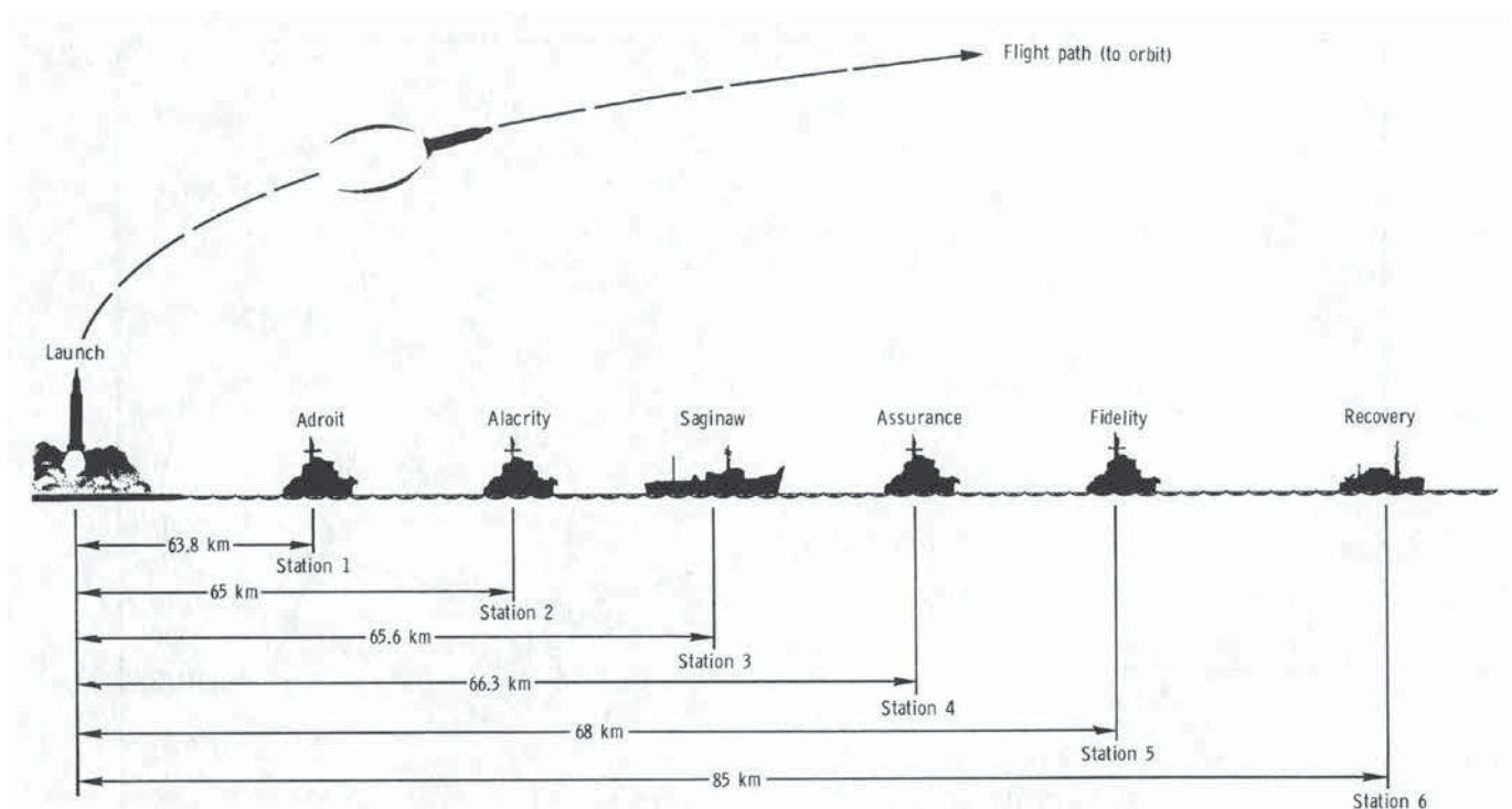
Figure 6.56. Schematic showing ship position for data acquisition during ascent (ref. 6.119).
