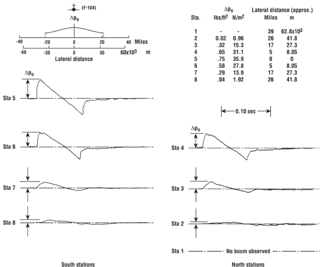
Figure 2.10. Measured sonic boom ground pressure signatures at several measuring stations at different distances to each side of the aircraft ground track. Airplane in steady-level flight at an altitude of 52,200 feet (15,911 m) and Mach 2: flight 3 (adapted from ref. 2.9).
