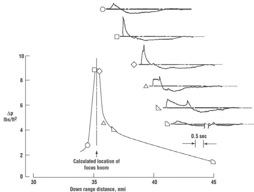
Figure 3.23. Saturn-Apollo 17 launch-ascent sonic boom signatures within focus region (ref. 3.39).
