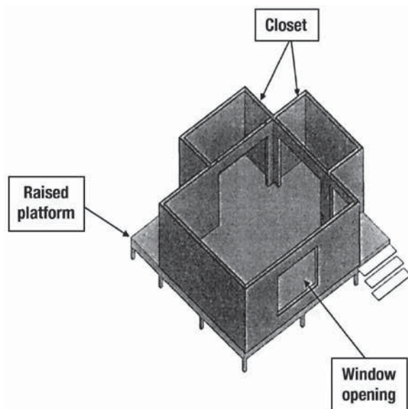
Figure 9.131. View of the structure of the simulator (ceiling has been removed for clarity, ref. 9.79).
