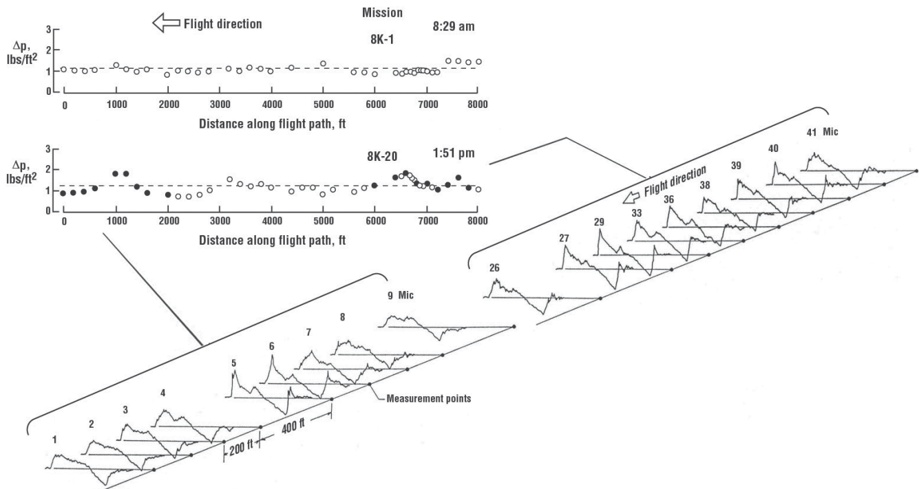
Figure 2.25. Variability in sonic boom overpressures and signature shapes of an F-104 aircraft flying above EAFB at Mach 1.3 and an altitude of 30,500 feet. This variability was measured along an 8000-foot array (adapted from ref. 2.24).
