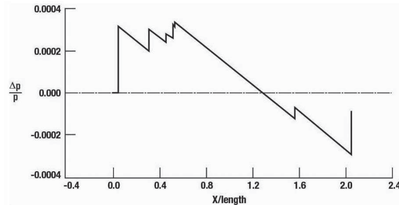
Figure 7.67. Baseline wing-body ground signature (adapted from ref. 7.28).
