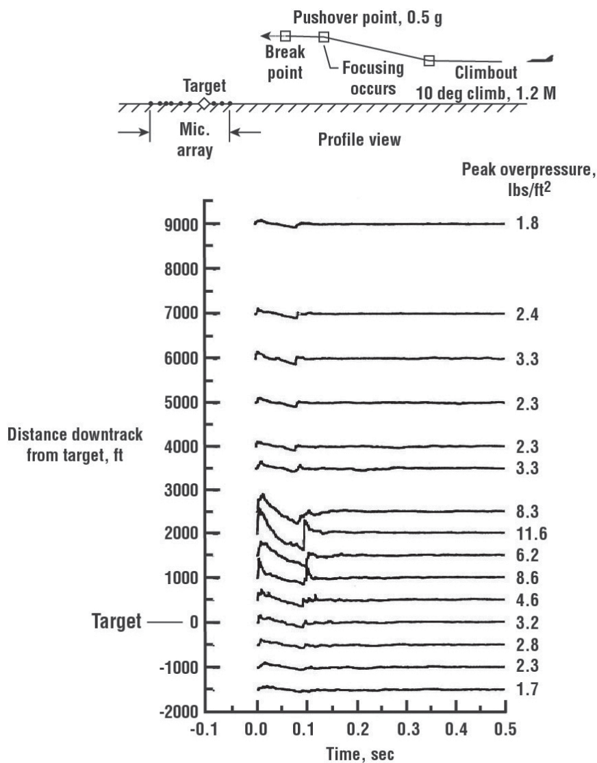
Figure 3.5. Measured sonic boom signatures from aircraft in -0.5\text{-g} climbout/pushover (adapted from ref. 3.6).
