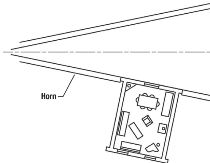
Figure 9.165. Psychoacoustic studies (ref. 9.95).
