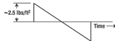
"Hybrid" waveform Cruise: Mach 1.7, 44,000 ft altitude
