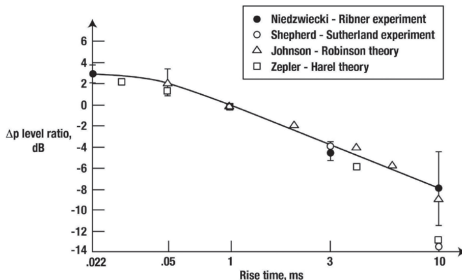
Figure 9.116. Equal loudness curve. Trade-off between overpressure level ratio ( -20 \log_{10} \Delta P_{\text{test}}/\Delta P_{\text{ref}} ) and rise time for 200 msec duration N-waves. \Delta P_{\text{ref}} = 1 \text{ lb/ft}^2 (48 Pa), t_{\text{ref}} = 1 \text{ msec} (ref. 9.65).
