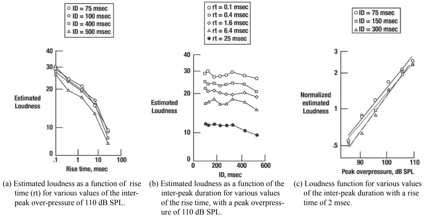
Figure 9.124. Results of the perceptual assessment of N-wave signals synthesized in the simulation room (adapted from ref. 9.69).
