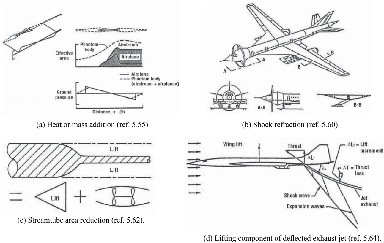
Figure 5.31. Some exotic concepts for boom minimization.
