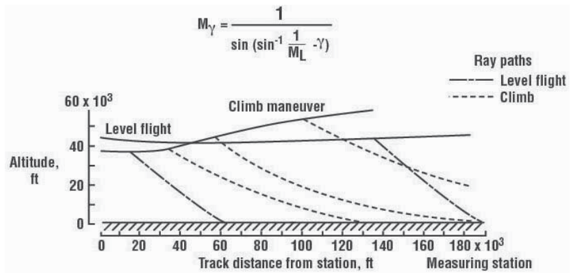
(c) Aircraft level and climb flight profiles and ray paths.
