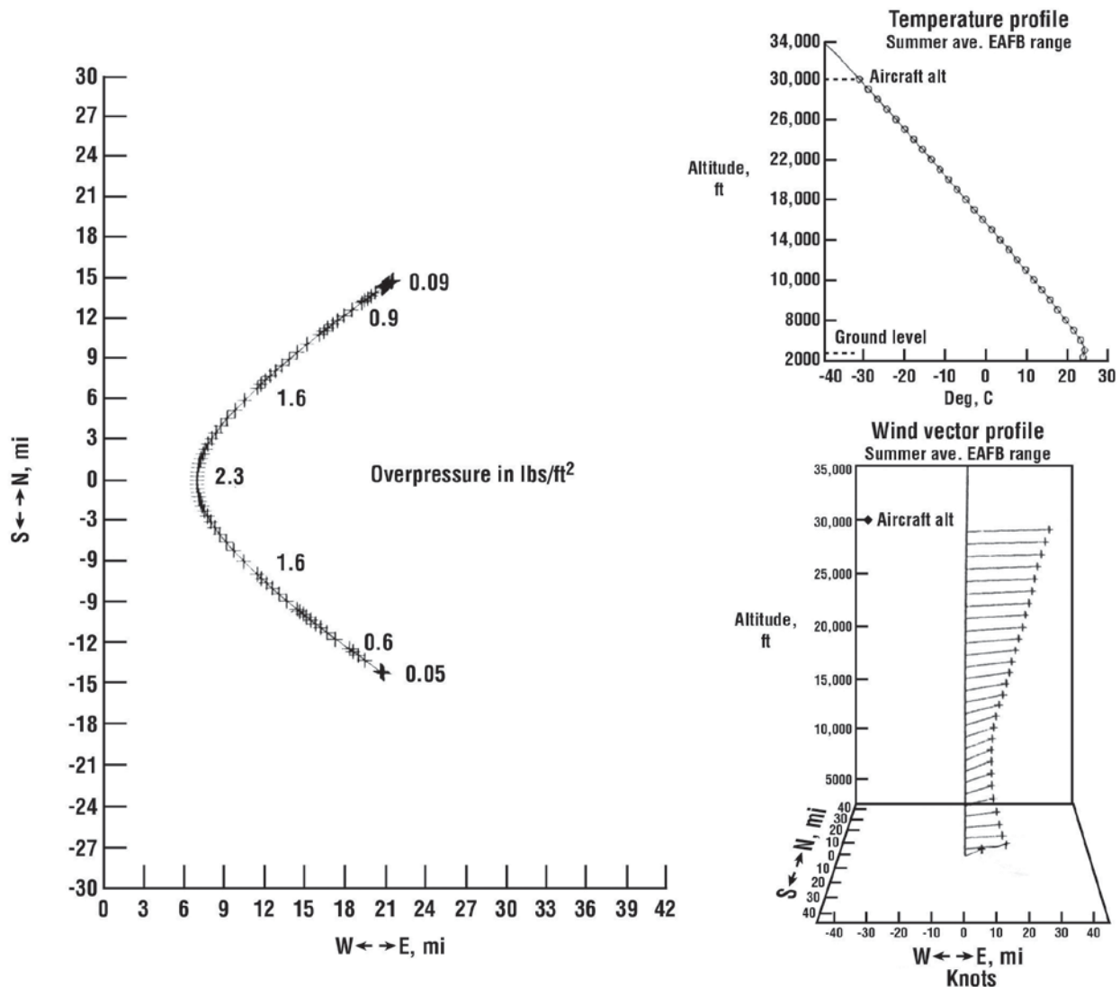
(a) F-111, Mach 1.34 steady at 30,000 feet MSL east-bound.
