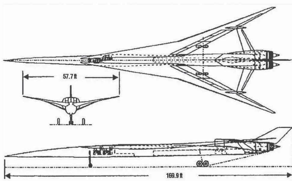
Figure 7.93. Dual-relevant vehicle (7.66).
