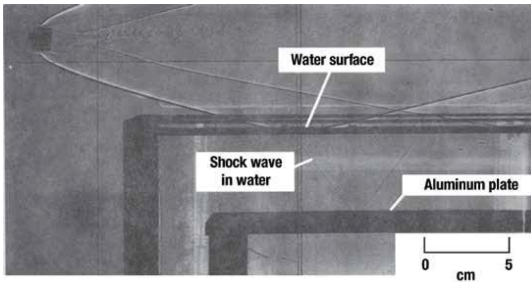
Figure 9.83. Shadowgraph pictures of model flying over Plexiglas water-filled tank at Mach 5.7 in air M_{\text{water}} = 1.3 (ref. 9.47).
