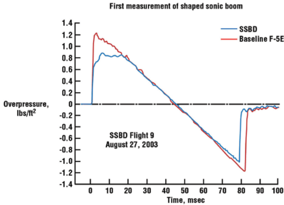
Figure 5.18. First measurement of a shaped sonic boom (ref. 5.37).
