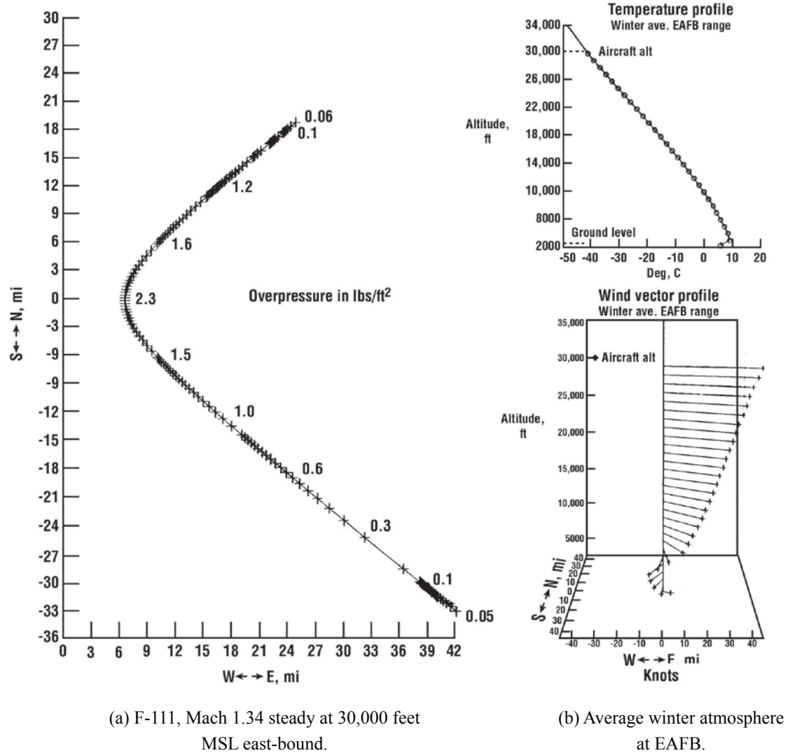
Figure 2.8. Winter atmospheric conditions and resulting sonic boom ground footprint for east-bound flight (adapted from ref. 2.5).
