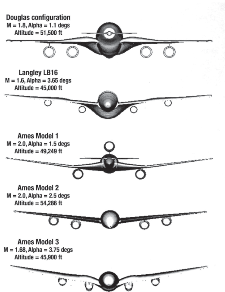
Figure 7.59. Front view of CFD geometry models for five low-boom aircraft (ref. 7.21).
