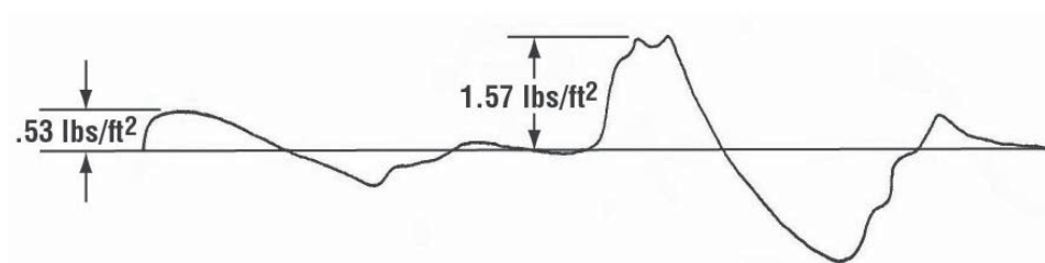
(c) Measured sonic boom pressure signature.
