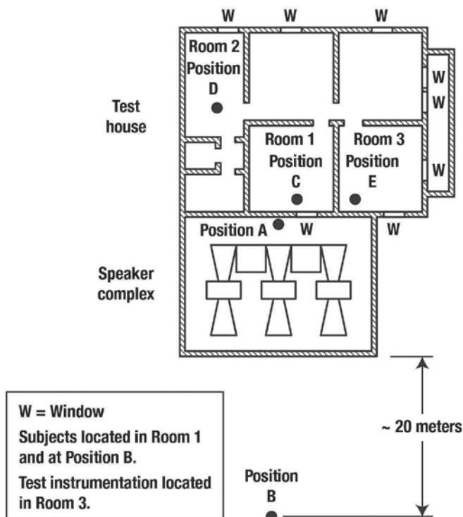
Figure 9.130. Layout of Georgia Tech simulator (ref. 9.77).
