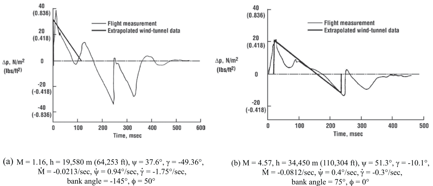
Figure 6.52. Apollo 15 Command Module wind-tunnel in-flight correlation (ref. 6.116).
